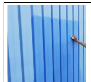
20 years old industrial facade painted metal profiles. Treated with: MPS REFRESH . After rubbing in twice.
